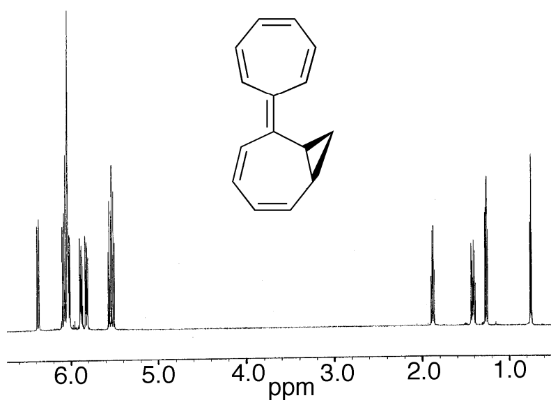
Fig. 600 MHz 1 H NMR Spectrum of 1,2-homoheptafulvalene (1).
